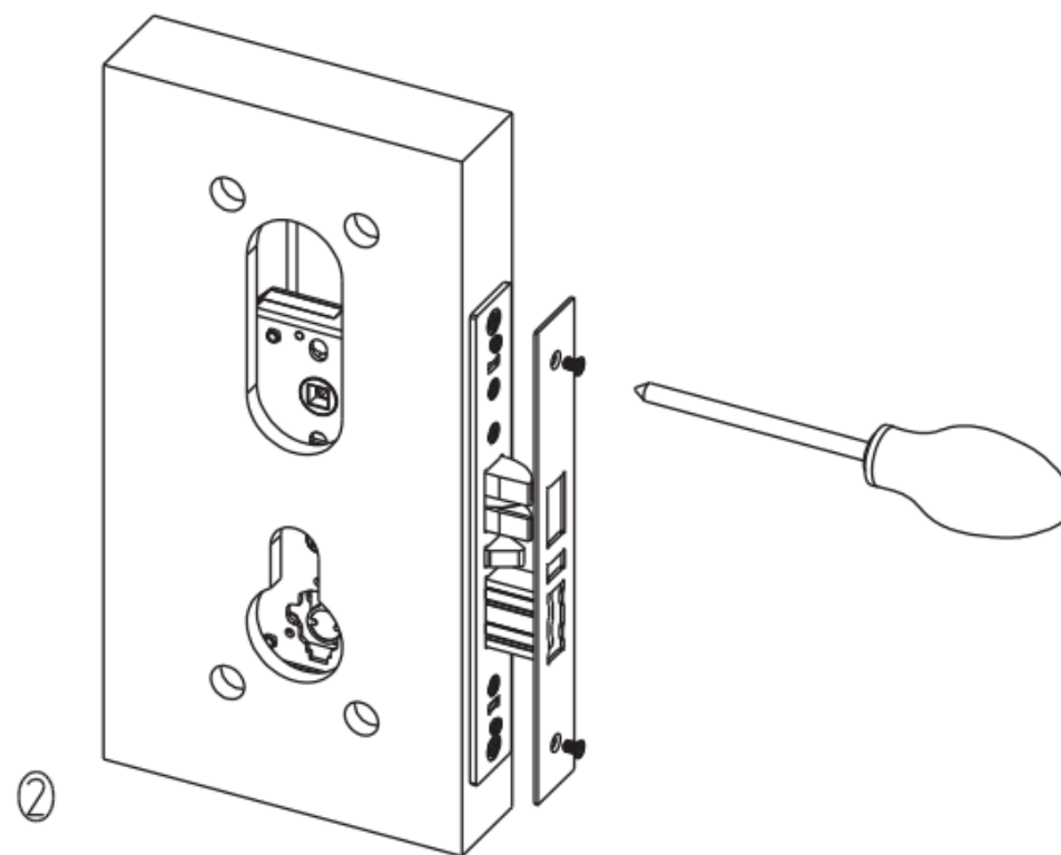
Pic(2) Mortise Faceplate
